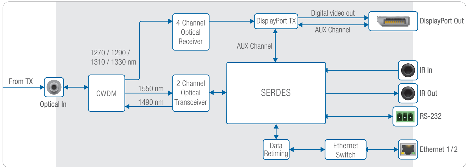
DVI-7380-RX Internal Block Diagram
